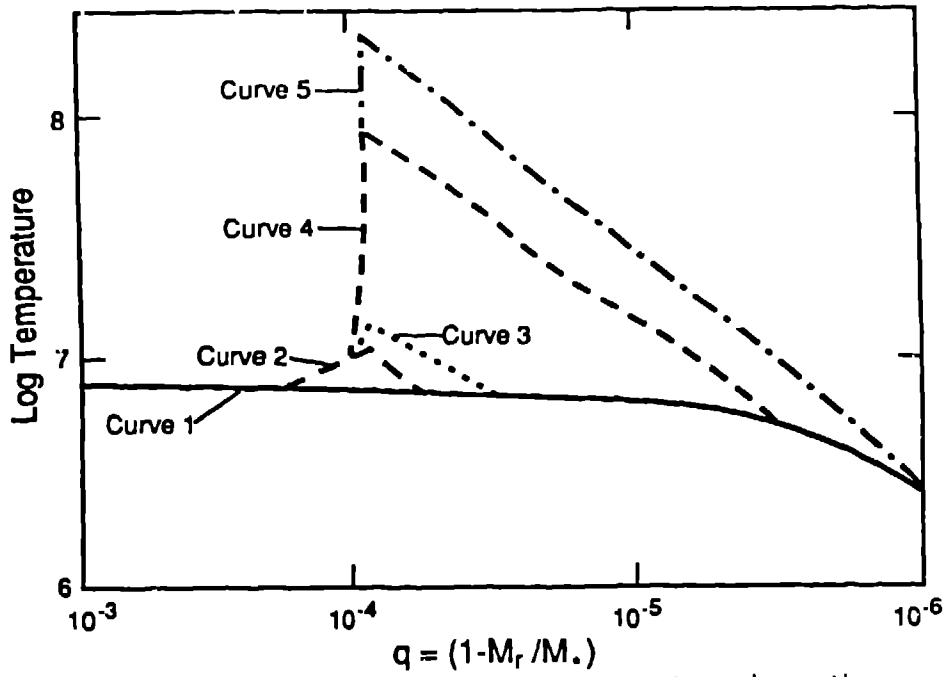
Fig. 1. Log temperature versus mass at various times during the TNR.
