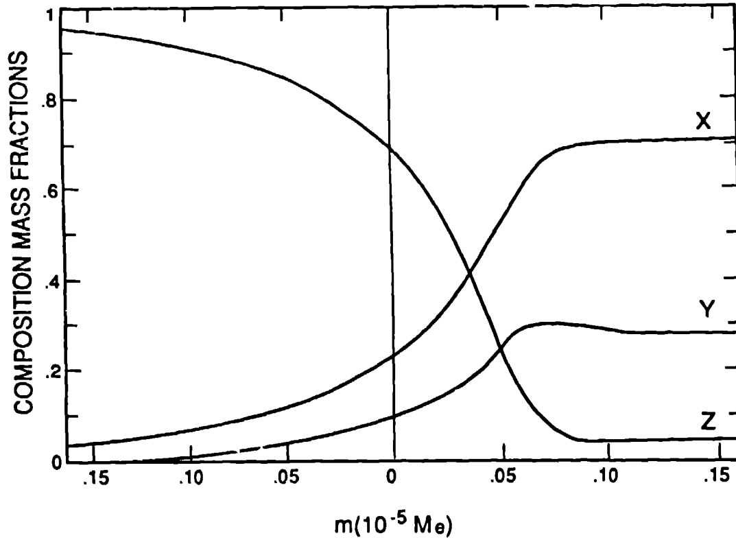
Fig. 7. Composition versus mass from Prialnik and Kovetz (1984).
