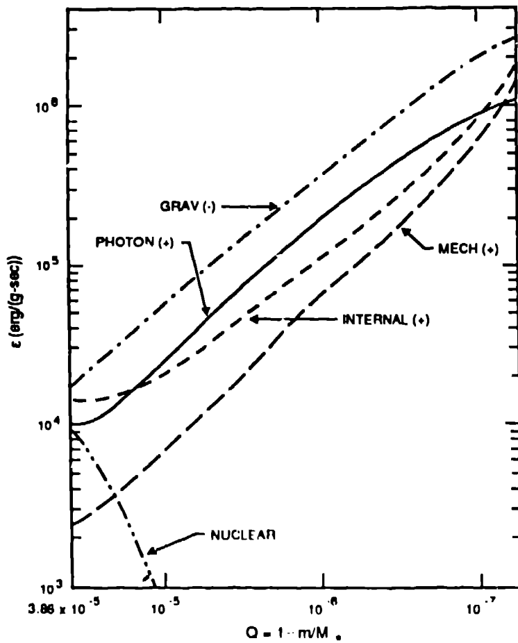
Fig. 2. Energy rates versus mass during the early stages of an accreting white dwarf.
