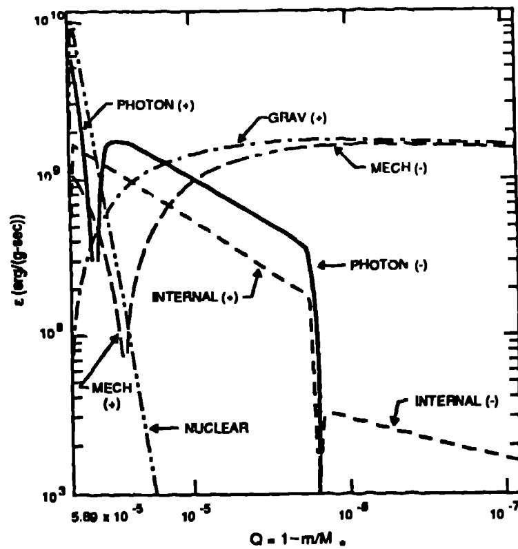
Fig. 3. Energy rates versus mass after the formation of a convective region on an accreting white dwarf.
